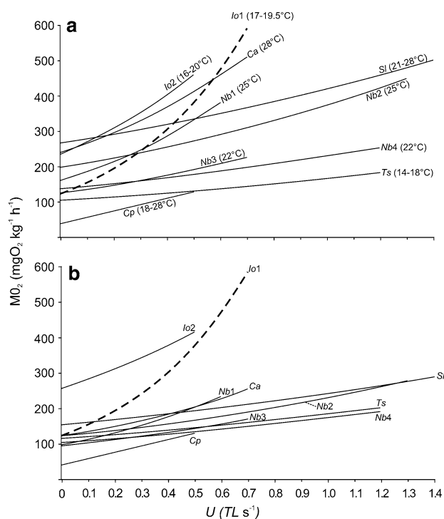
Fig. 3 Measured oxygen consumption plotted versus relative swim speed, U (TL) s^{-1} for sharks at a respective experimental temperatures and b corrected to 18°C. Io1 ( Isurus oxyrinchus , shortfin mako) n = 9 (this study); Io2 ( I. oxyrinchus ) n = 1 , 3.2 kg (adapted from Graham et al. 1990); Ca ( Carcharhinus acronotus , blacknose shark) n = 8 , 0.4–3.5 kg (adapted from Carlson et al. 1999); Nb1 ( Negaprion brevirostris , lemon shark) n = 7 , 0.8–1.3 kg (adapted from Scharold and Gruber 1991); Sl ( Sphyrna lewini , scalloped hammerhead) n = 17 , 0.5–0.9 kg (adapted from Lowe 2001, uncorrected raw data); Nb2 ( N. brevirostris ) combined data for n = 1 , 1.65 kg (adapted from Graham et al. 1990) and n = 7 , 0.8–1.3 kg (adapted from Scharold and Gruber 1991); Nb3 ( N. brevirostris ) n = 13 , 0.8–1.3 kg (adapted from Bushnell et al. 1989); Nb4 ( N. brevirostris ) combined data for n = 1 , 1.65 kg (adapted from Graham et al. 1990) and n = 13 , 0.8–1.3 kg (adapted from Bushnell et al. 1989); Ts ( Triakis semifasciata , leopard shark) n = 5 , 2.2–5.8 kg (adapted from Scharold et al. 1989); Cp ( Carcharhinus plumbus , sandbar shark) n = 16 , 1.0–10.3 kg (adapted from Dowd et al. 2006; 6.8 kg)
