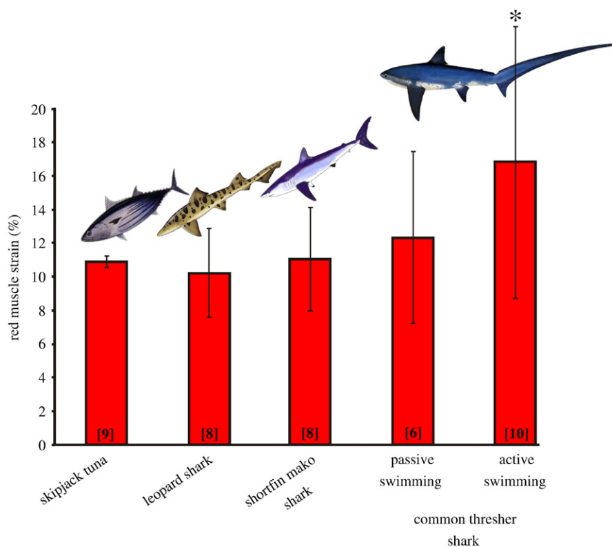
Fig. 3. Red muscle strain amplitude (peak-to-peak) during active swimming in select species of fish. Data for passive swimming is also presented for the common thresher shark. *indicates significant difference between active and passive swimming. Values are mean \pm SD and sample size. Data for skipjack tuna ( Katsuwonus pelamis ), a thunniform swimmer with medial RM, from Shadwick et al. (1999), shortfin mako shark ( Isurus oxyrinchus ), a thunniform swimmer with medial RM, from Donley et al. (2005), and leopard shark ( Triakis semifasciata ), a subcarangiform swimmer with subcutaneous RM, from Donley and Shadwick (2003).
