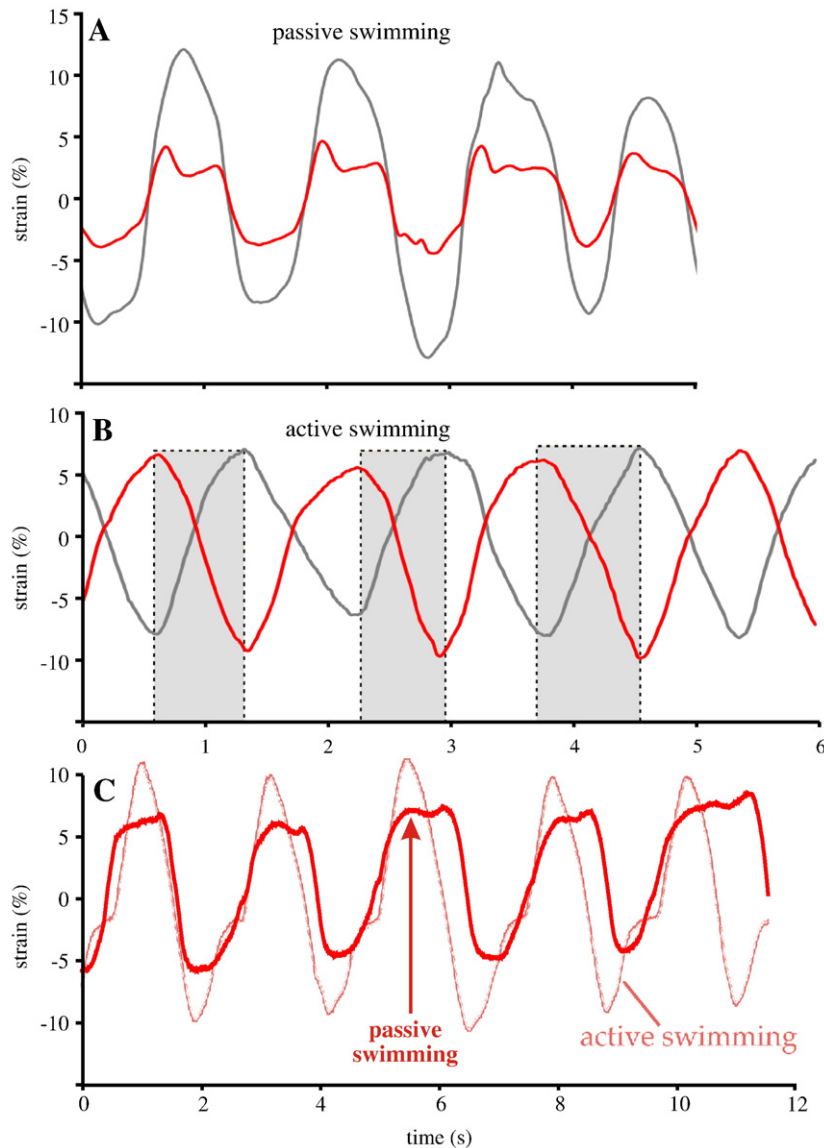
Fig. 2. Trajectories of red muscle (red-line) and white muscle (grey-line) strain during active and passive swimming in common thresher sharks. A) During passive swimming strain of RM and WM are in phase, whereas B) during active swimming in the same fish the strain trajectories are out of phase. Shaded boxes indicate the degree of phase shift (i.e., peak RM strain to peak WM strain). C) Comparison of strain trajectories of RM from another individual during active (fine trace) and passive swimming (bold trace), illustrating the prominent double peak often observed during passive swimming (see also panel A).
