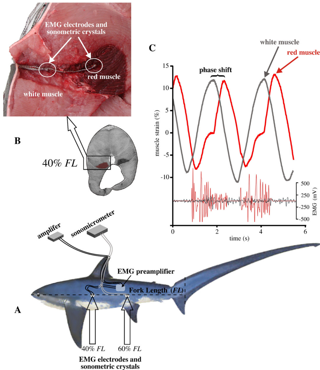
Fig. 1. A) Thresher shark showing the two positions along the length of the body (i.e., 40 and 60% fork length, FL , dashed line) where pairs of sonomicrometry crystals and EMG leads were implanted into the medial red (RM) and overlying white myotomal muscles (WM). Preamplified EMG signals and sonomicrometry cables were connected to amplifiers and the sonomicrometer on board the vessel. B) Transverse section of a thresher shark at 40% FL showing the position of sonomicrometer crystals and EMG leads in the RM and WM. A second pair of crystals was located about 15 mm posterior to these (not shown). C) RM and WM strain recorded with sonomicrometry, illustrating the amplitude and phase shift between the muscles. EMG records during cruise swimming showing activity in RM but not in WM.
