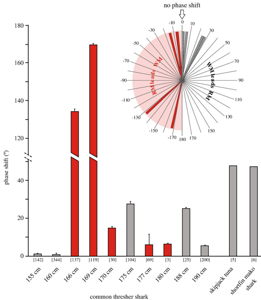
Fig. 4. Phase shift between peak of red (RM) and white muscle (WM) strain trajectories (see Fig. 1C) in the common thresher sharks during active cruise swimming. Phase shift expressed as degrees of the tail-beat cycle in a linear scale and on a circular plot (inset). Instances in which the WM leads the RM are shown in grey, and where RM leads the WM are shown in red. The fork length of each individual thresher shark is noted below the bars and values are mean \pm SE and sample size. Data for skipjack tuna ( Katsuwonus pelamis ) from Shadwick et al. (1999) and for mako shark ( Isurus oxyrinchus ) from Donley et al. (2005). Detailed morphometric data for each individual thresher shark in the inset are given in Table 1.
